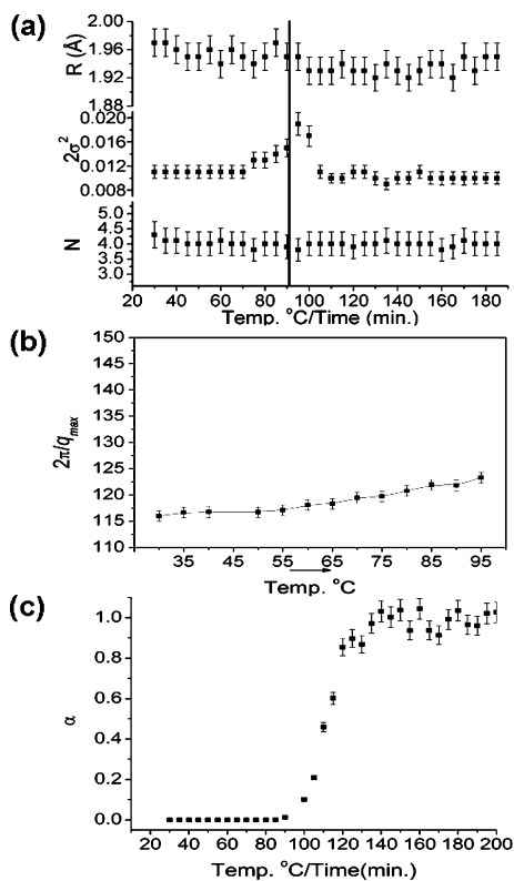
Figure 3. Analysis of the data presented in Figure 2: (a) Zn–O EXAFS data, (b) change of 2\pi/q_{\max} position, and (c) extent of crystallization obtained from the reflection intensity change in the WAXS. The increase in the Debye–Waller factor at the onset of crystallization (illustrated by the black line in (a)) is probably artificial and due to fluctuations in sample density as the sample moves in the hydrothermal vessel.
