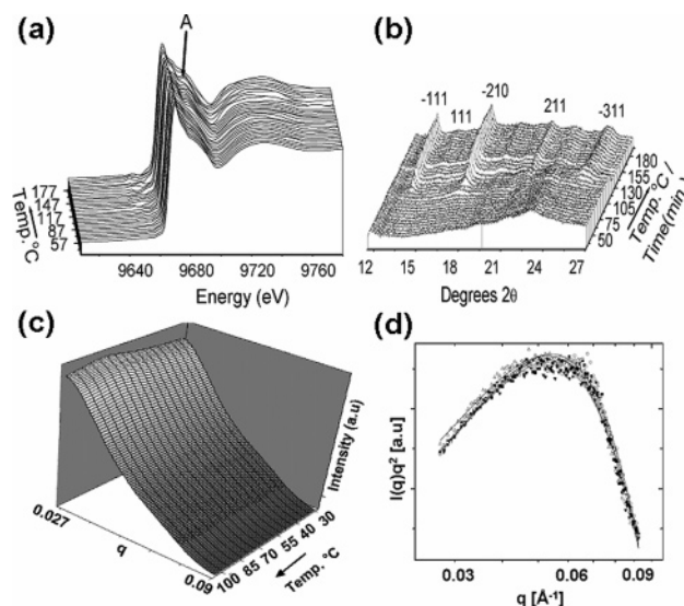
Figure 2. In situ XANES with arrow marking the multiple scattering feature at ~9.685 keV (a), WAXS with reflections indexed to CHA (b), raw SAXS data (c), and I(q) \times q^2 - \log(q) plots (Kratky type plot) (d) from the SAXS data collected during crystallization.
